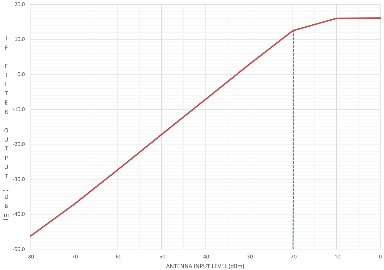
Express Receiver Front End Gain Compression Characteristic (14,175-KHz)
